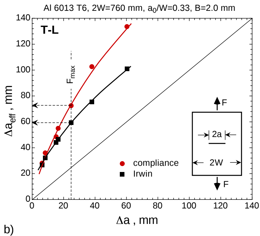
Figure 4.32: Comparison between effective crack extensions, \Delta a_{\text{eff}} , according to the compliance method and Irwin correction plotted versus physical crack extension, \Delta a , measured from the side surface. a) L-T and b) T-L orientations.
