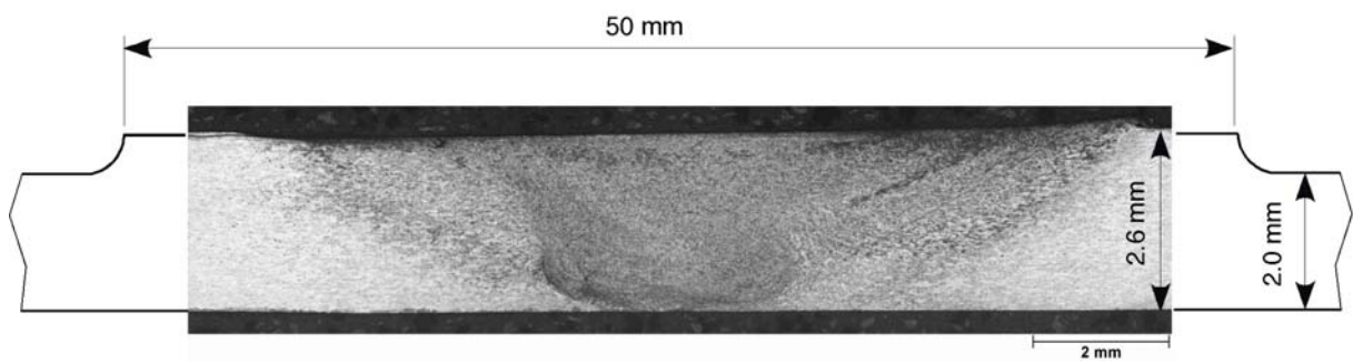
FSW butt-joint
