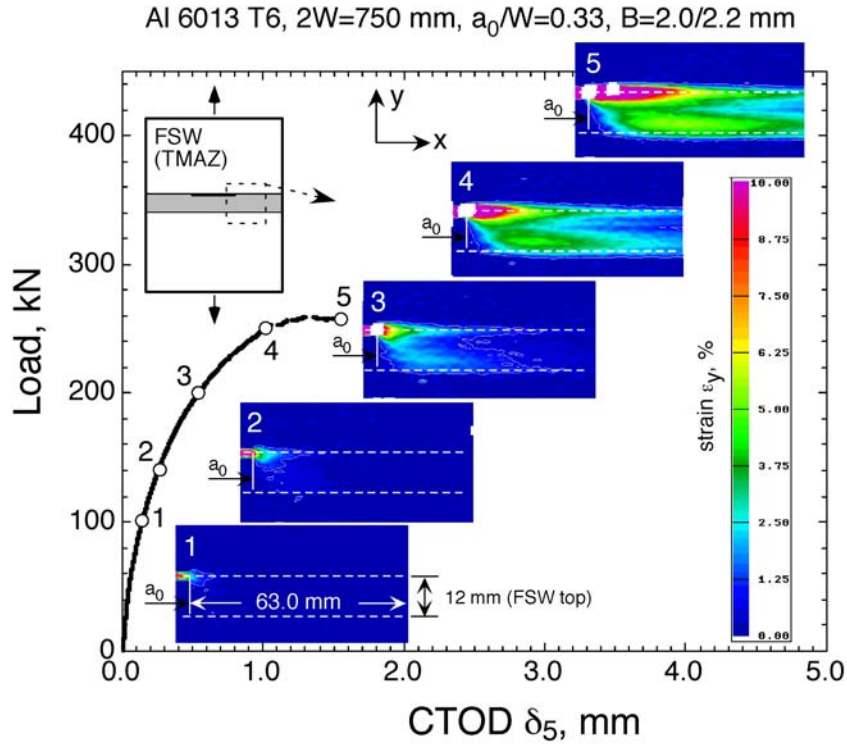
Figure 4.55: Evolution of the plastic zone ahead of the crack tip in the M(T)750 FSW plate with a crack in TMAZ.
