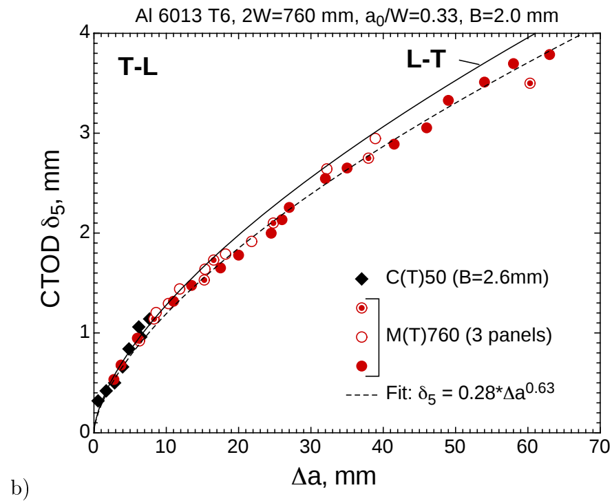
Figure 4.34: CTOD \delta_5 R-curves of the base material. a) L-T and b) T-L orientations.
