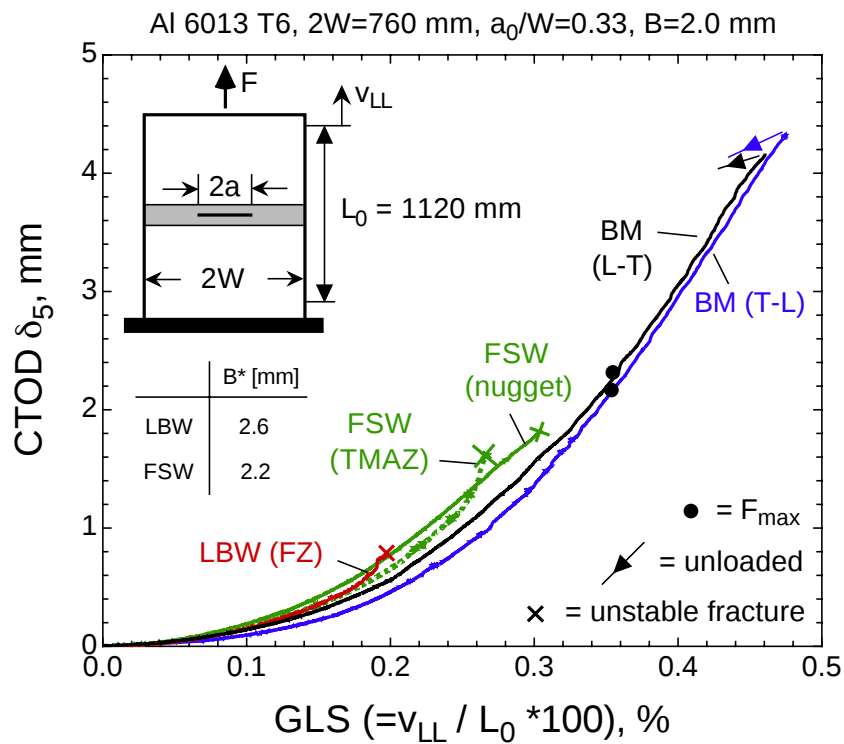
Figure 4.26: Comparison of CTOD \delta_5 vs. the gauge length strain (GLS) curves for base material (BM) and welded (LBW and FSW) panels.
