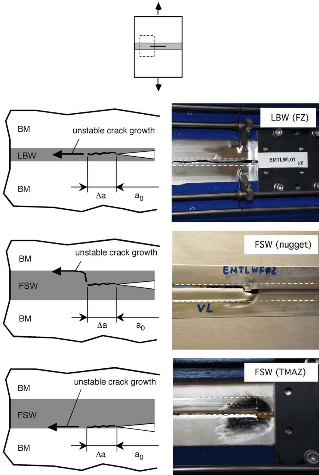
Figure 4.27: Fracture path of welded panels. All welded panels exhibited a small amount ( \sim 4\text{-}9\text{ mm} ) of stable crack extension, \Delta a , prior to an unstable fracture. In the FSW panel (FSW(nugget)), the crack located in the nugget zone stably grew along the weld centerline and finally deviated into the TMAZ during the unstable fracture.
