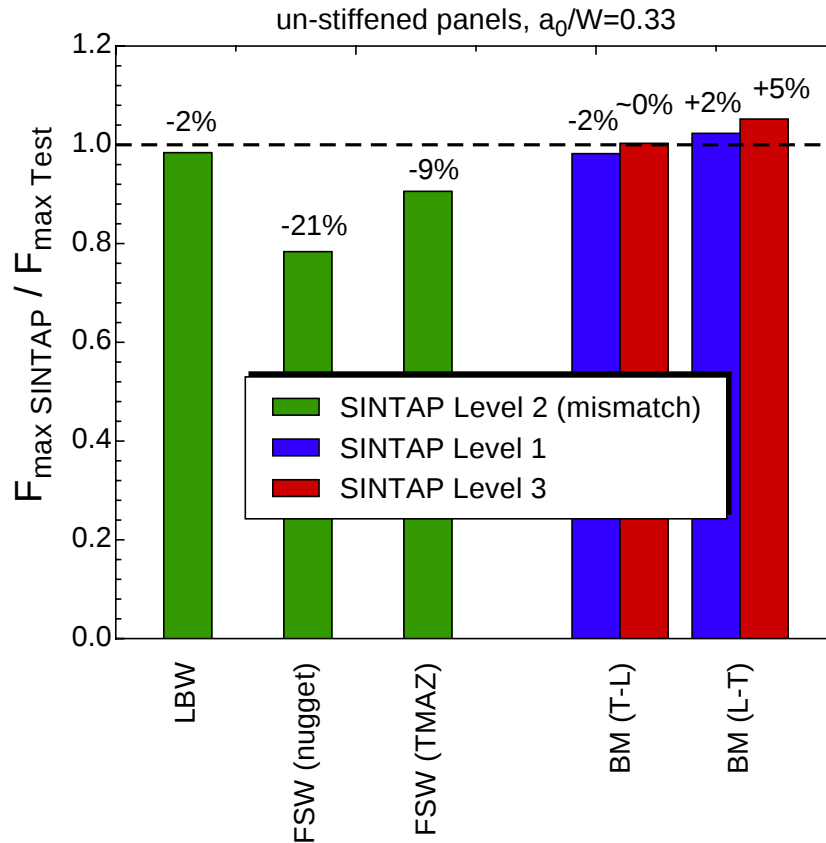
Figure 6.15: Summary of residual strength predictions with the SINTAP procedure for unstiffened cracked base material (BM), LBW and FSW (crack in the nugget area and TMAZ) panels.
