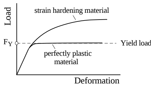
Figure 5.12: Definition of the yield load.
