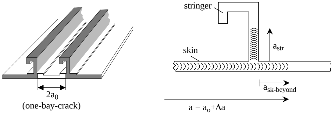
Figure 5.3: Crack branching.
