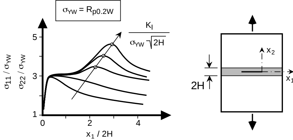
Figure 2.15: Stress distribution along the ligament for different loading levels [30]. Results of an FE large deformation analysis based on an elastic base and elastic-plastic weld material model with strain hardening. \sigma_{YW} denotes the yield strength of the weld material.
