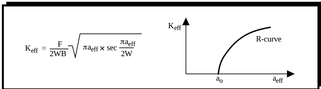
Figure A.4: Determination of the R-curve according to the compliance method of the ASTM E561 standard [16].
