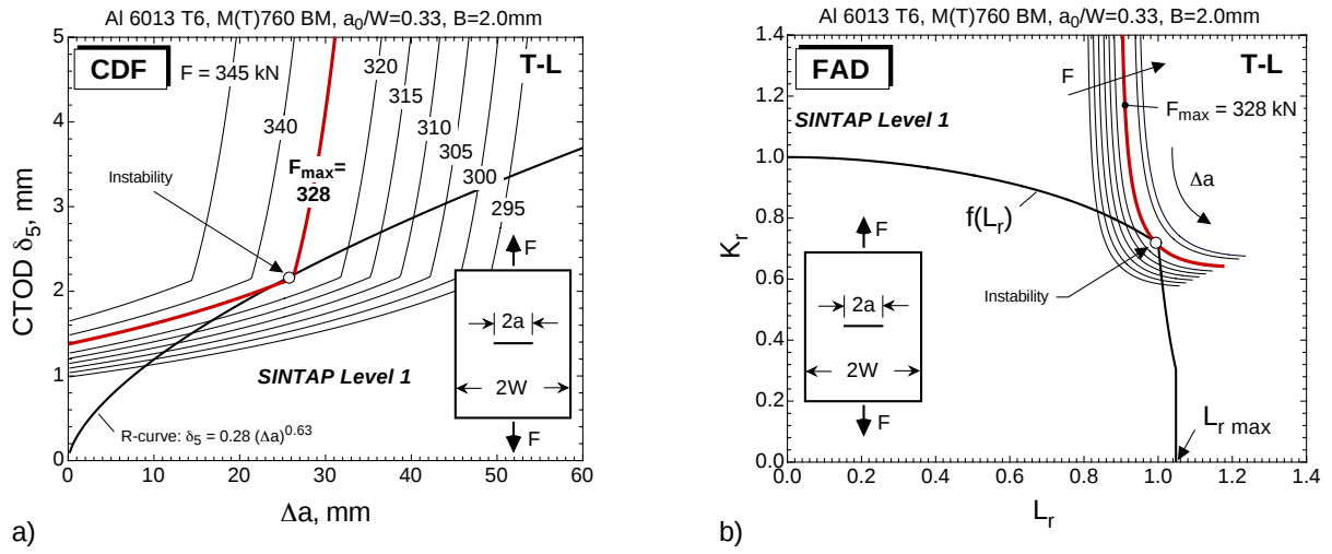
Figure A.9: Residual strength prediction of the base material (T-L orientation) panel using a) CDF and b) FAD approaches of the SINTAP procedure. Analysis Level 1 is based on the CTOD \delta_5 R-curve showing the equivalence of the two methods. Crack driving forces in the FAD approach are calculated for the same loads as in the CDF approach.
