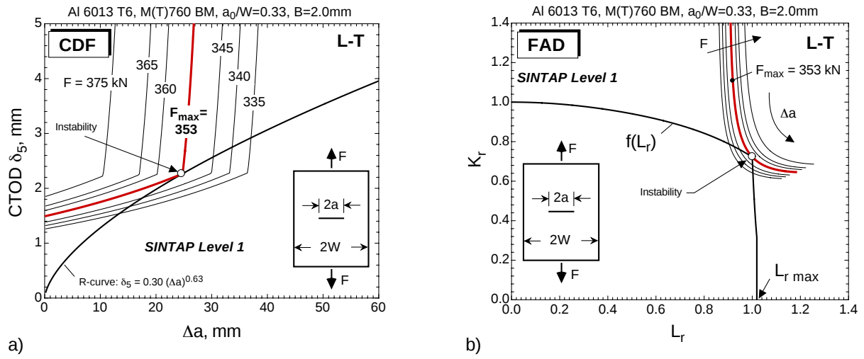
Figure A.11: Residual strength prediction of the base material (L-T orientation) panel using a) CDF and b) FAD approaches of the SINTAP procedure. Analysis Level 1 is based on the CTOD \delta_5 R-curve showing the equivalence of the two methods. Crack driving forces in the FAD approach are calculated for the same loads as in the CDF approach.
