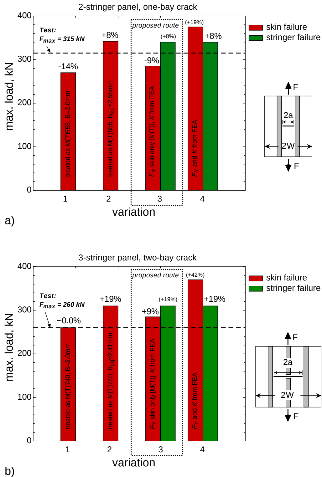
Figure 6.31: Summary of the residual strength predictions for a) 2-stringer welded stiffened panels with a one-bay crack and b) 3-stringer welded stiffened panel with a two-bay crack. The variations of the K -factor and yield load solutions are given in Tab. 6.7 for the 2-stringer panel and in Tab. 6.8 for the 3-stringer panel.
