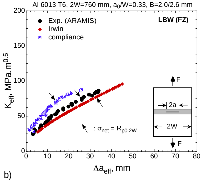
Figure 4.57: a) Comparison between theoretical (Irwin and compliance) and experimental (ARAMIS) plastic zone sizes in the M(T)760 LBW panel. b) Respective K_{\text{eff}} R-curves where \Delta a_{\text{eff}} = r_p .
