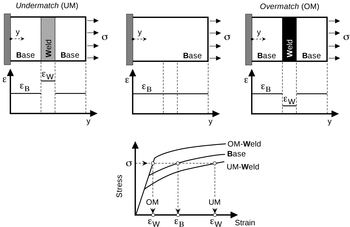
Figure 2.10: Strength mismatch phenomenon for a welded panel loaded transverse to the weld direction. \varepsilon_B and \varepsilon_W denote the strain in the base and weld materials, respectively.
