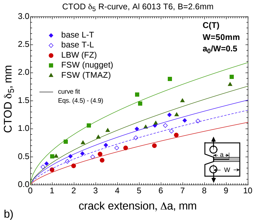
Figure 4.9: a) Load versus CTOD \delta_5 plot for base material and welded joints. b) CTOD \delta_5 R curves for the base material and welded joints.
