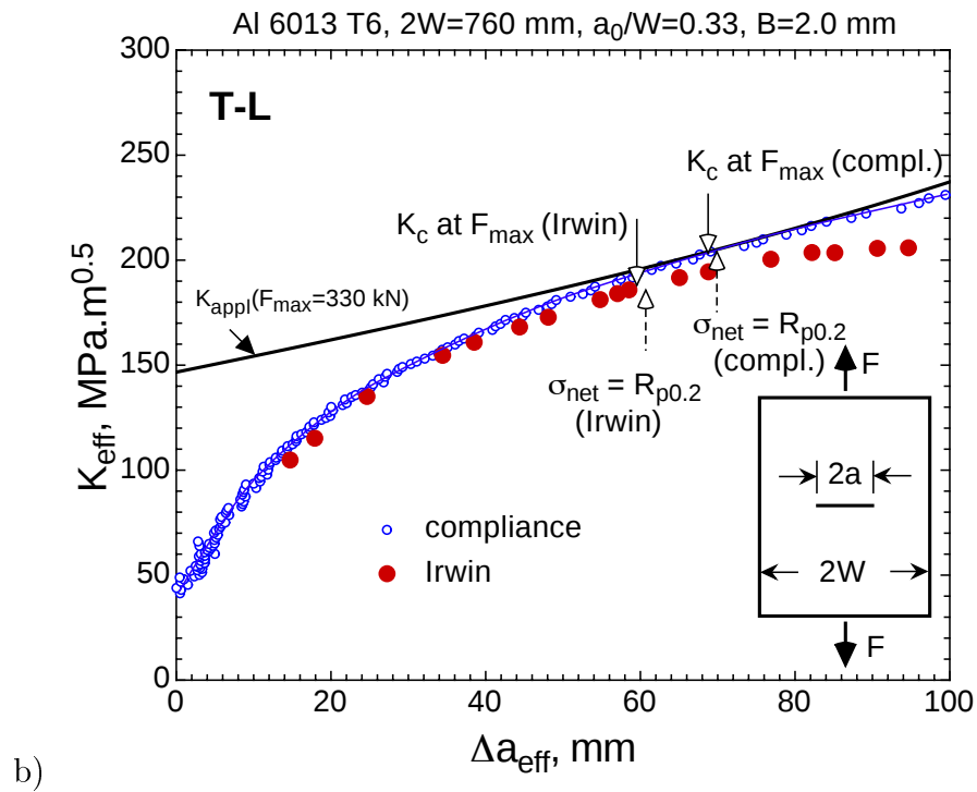
Figure 4.30: K_{\text{eff}} R-curves of the base material. a) L-T and b) T-L orientations.
