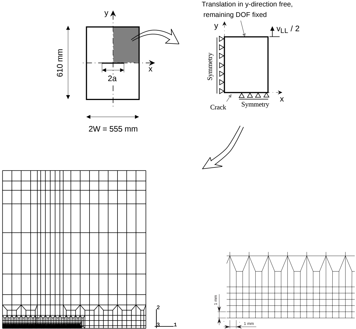
Figure 5.6: FE mesh of the M(T) panel (one quarter due to symmetry).
