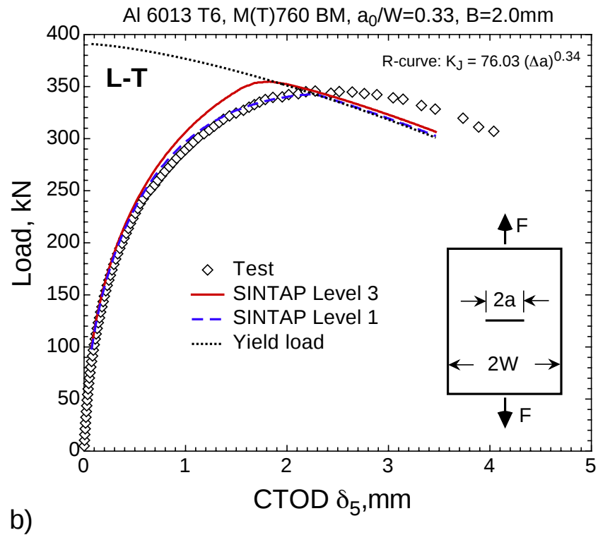
Figure 6.6: Comparison between SINTAP predictions and experimental results for the base material panels in L-T orientation. Analysis is based on the K_J R-curve. a) load- \Delta a curve; b) load-CTOD \delta_5 curve.
