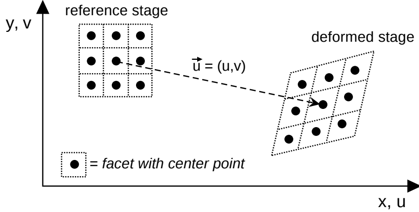
Figure 4.45: 3 \times 3 environment for the strain calculation. The dots indicate the center of a facet. The strain is determined at the center of the middle facet by including the eight adjacent facets.
