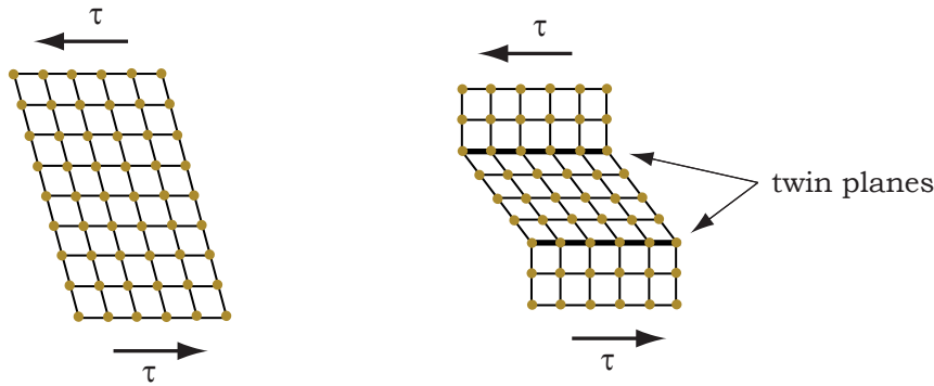
Figure 2.4: Crystal lattice reorientation due to mechanical twinning
