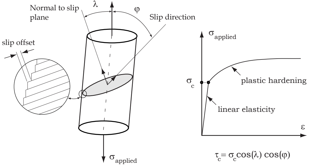
Figure 2.3: Relationship between applied stress \sigma_{applied} and shear stress \tau acting on a specific slip system in a uniaxial tensile test
