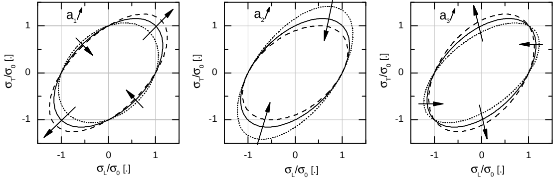
Figure 8.1: Influence of model parameters a_i onto the yield surface shape. \sigma_0 is the yield stress for uniaxial tension in L -direction. Continuous line represents von Mises yield locus ( a_i = 1 and b_i = 0 )
