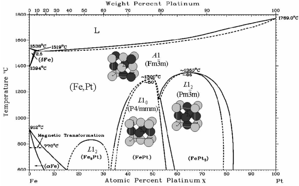
Figure 2.1.: Phase diagram of the \text{Fe}_{100-x}\text{Pt}_x system with the corresponding crystallographic structures [36] in dependence of the temperature. L, A1, L1_0 and L1_2 are the strukturbericht symbols for the different crystal structures (adapted from [37]).
