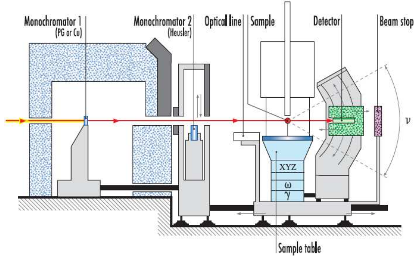
Figure 4.6.: Side view of the diffractometer D23 at ILL (adapted from [84]). The monochromator 2 is only used for polarized measurements.
