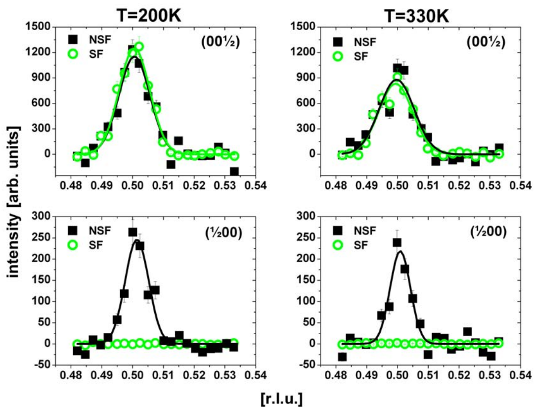
Figure 5.21.: Polarization analysis of the \text{Fe}_{50}\text{Pt}_{32.5}\text{Rh}_{17.5} film for the half order (00\frac{1}{2}) and (\frac{1}{2}00) reflection at T=200\text{K} and T=330\text{K} . The guide field was directed along the [010] -direction (b-axis) of the film.
