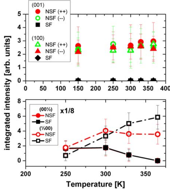
Figure 5.25.: Polarization analysis of the Fe 50 Pt 25 Rh 25 film for the nuclear Bragg reflections (001), (100) and the AF (00 \frac{1}{2} ), ( \frac{1}{2} 00) peaks. Plotted are the integrated intensities (including the data treatment) against the temperature. The integrated intensity of the (00 \frac{1}{2} ) reflection has been multiplied by a factor 1/8.
