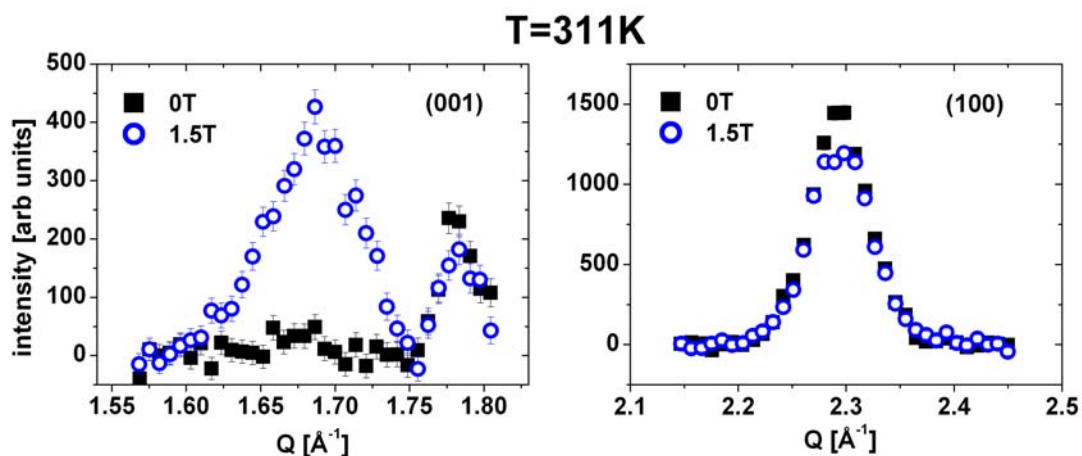
Figure 5.34.: Magnetic field dependence of the (001) and (100) reflection of the \text{Fe}_{50}\text{Pt}_{45}\text{Rh}_5 film at T=311\text{K} for 0 T (black squares) and 1.5 T (open circles). The magnetic field was directed along the a-axis.
