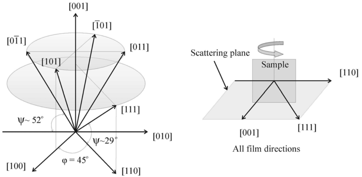
Figure 5.3.: Orientation of the different sample directions and the orientation of the scattering plane (adapted from [76]).
