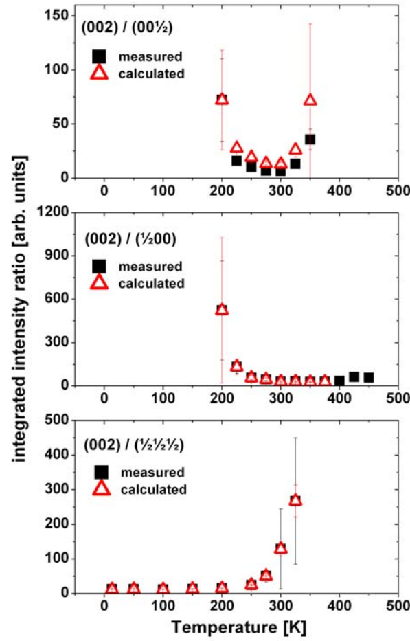
Figure 5.54.: Integrated intensity ratios of the (002) reflection and the (00\frac{1}{2}) , (\frac{1}{2}00) and (\frac{1}{2}\frac{1}{2}\frac{1}{2}) reflection for the measured data (black squares) and the ratios calculated for the model of the \text{Fe}_{50}\text{Pt}_{25}\text{Rh}_{25} film (red open triangles).
