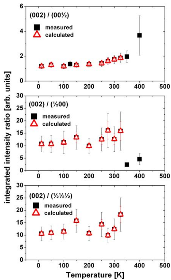
Figure 5.48.: Integrated intensity ratios of the (002) reflection and the (00\frac{1}{2}) , (\frac{1}{2}00) and (\frac{1}{2}\frac{1}{2}\frac{1}{2}) reflection for the measured data (black squares) and the ratios calculated for the model of the \text{Fe}_{50}\text{Pt}_{32.5}\text{Rh}_{17.5} film (red open triangles).
