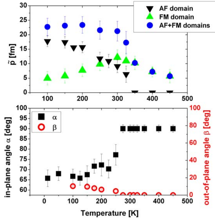
Figure 5.50.: Temperature dependence of the magnetic scattering length \tilde{p}(T) [upper panel] and the in-plane and out-of-plane angles \alpha and \beta [lower panel] of the \text{Fe}_{50}\text{Pt}_{40}\text{Rh}_{10} film. Note: only the angles of the AF domain are shown since in the FM domain all magnetic moments are oriented in the out-of-plane direction ( \beta = 90^\circ ).
