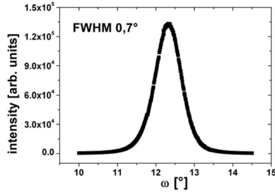
Figure 5.2.: Rocking scan of the (001) reflection of the \text{Fe}_{50}\text{Pt}_{32.5}\text{Rh}_{17.5} film.
