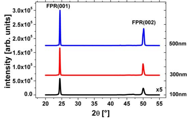
Figure 5.8.: Comparison of the out-of-plane X-ray diffraction scans of the Fe 50 Pt 40 Rh 10 (FPR) films for different sample thicknesses. The intensity of the 100nm film was multiplied by a factor of 5.
