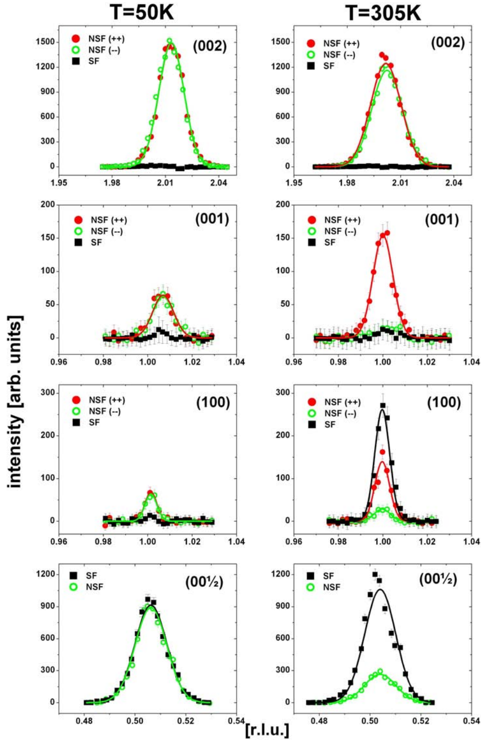
Figure 5.39.: Polarization analysis of the 500 nm \text{Fe}_{50}\text{Pt}_{40}\text{Rh}_{10} film for the (002), (001), (100) and (00\frac{1}{2}) reflection at T=50\text{K} and T=305\text{K} within an applied field of 1 T.
