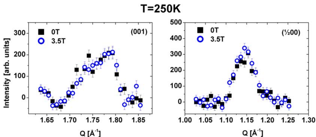
Figure 5.35.: Magnetic field dependence of the (001) and (\frac{1}{2}00) reflection of the \text{Fe}_{50}\text{Pt}_{32.5}\text{Rh}_{17.5} film at T=250\text{ K} for 0 T (black squares) and 3.5 T (open circles). The magnetic field was directed in-plane along the b-axis.
