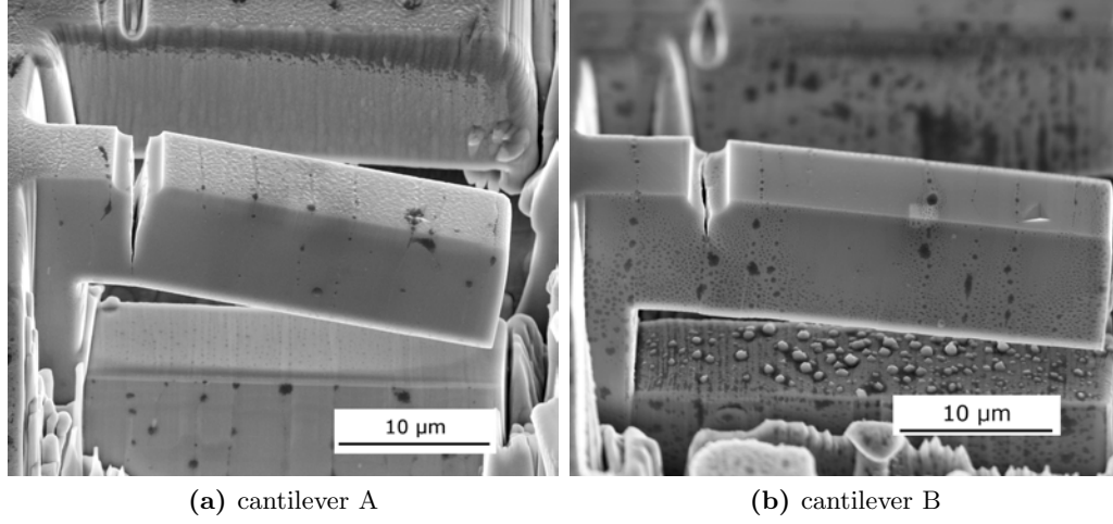
Figure 6.10 Cantilevers showing fracture (a) directly after the onset of plastic deformation and (b) after pronounced plastic deformation.
