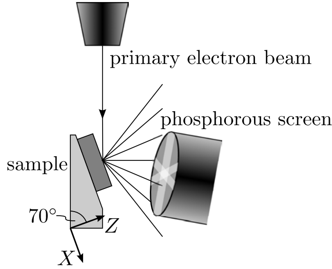
Figure 3.3 Schematic representation of an EBSD system.
