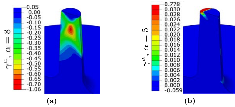
Figure 5.8 Simulation of a deformed column (CC-1) shown in figure 5.2. The color code represents the shear strain, \gamma , (a) on the slip system with the highest Schmid factor, 0.48, and (b) the slip system providing the second highest Schmid factor, 0.40.
