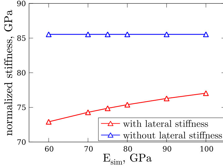
Figure 4.10 Normalized stiffness as a function of the elastic modulus chosen for the simulation for a laterally unconstrained and a laterally constrained indenter.
