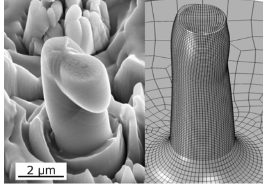
Figure 5.7 Comparison of the deformations of a tested specimen (CC-1) and the corresponding simulation. The simulation depicts the result corresponding to 10 % nominal strain while the maximum nominal strain in the experiment was 30 %. The slip direction in the experiment is identical to the slip direction in the simulation.
