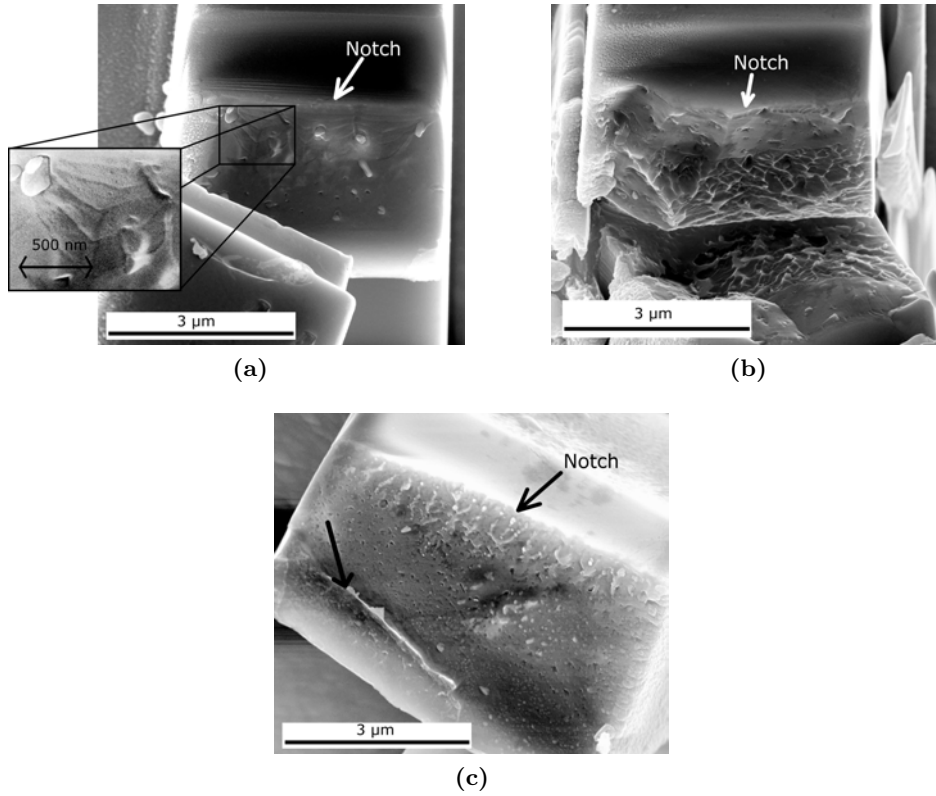
Figure 4.15 (a) Smooth fracture surface of a grain boundary in an underaged specimen showing large particles and striation like lines. (b) Partially dimpled fracture surface of an underaged specimen. (c) fracture surface of a grain boundary in a peak-aged specimen with finely distributed particles, the arrow marks the position where the crack stopped.
