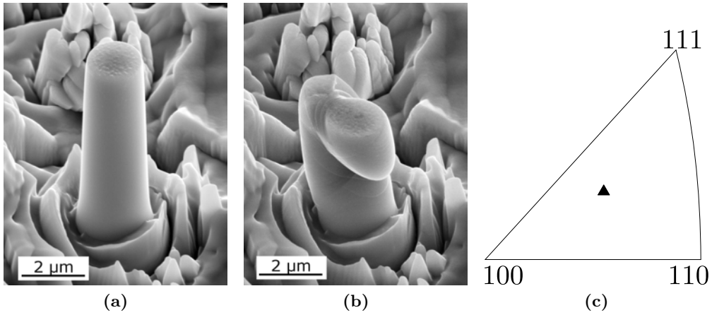
Figure 5.2 Example for a micro-column (a) before and (b) after the compression experiment. (c) Inverse pole figure describing the orientation of the compression axis in relation to the grain.
