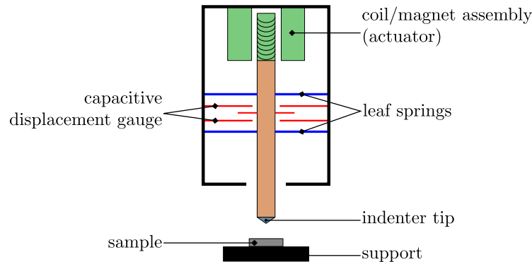
Figure 3.2 Schematic representation of a nanoindentation head.
