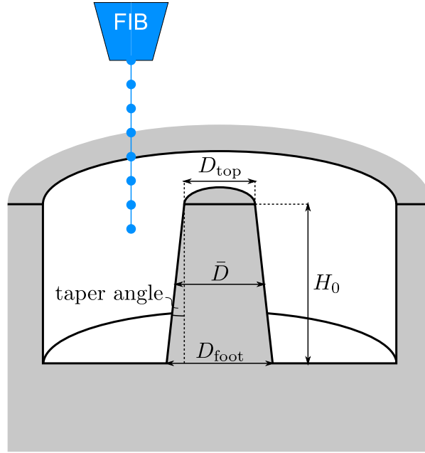
Figure 5.1 Annular milling procedure for the fabrication of micro-columns. The column geometry is determined by the initial height, H_0 , and the diameter at the top, D_{\text{top}} , and at the foot, D_{\text{foot}} , of the column. The average diameter, \bar{D} , and the taper angle are calculated assuming that the diameter increases linearly from the top to the foot.
