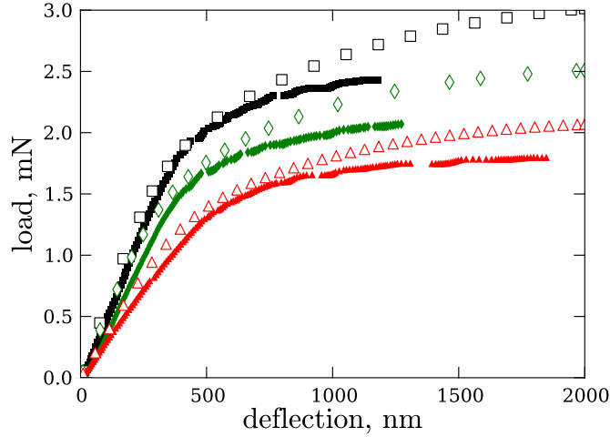
Figure 6.3 Comparison of the experimental load-deflection response of three cantilevers with a grain boundary under the notch (solid symbols) with the corresponding simulation data (open symbols).
