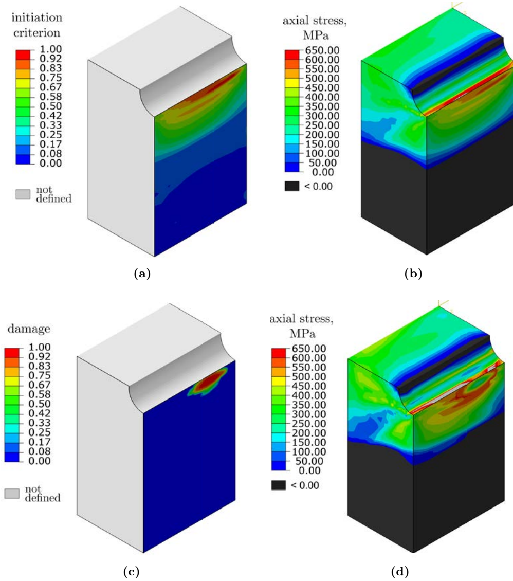
Figure 6.15 Cantilever B: (a) Initiation criterion and (b) stress distribution at the grain boundary at the moment of initiation. (c) Damage and (d) normal stress distribution at the grain boundary for the last increment of the simulation.
