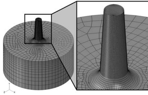
Figure 5.5 Example FE-mesh for modeling of the deformation of a micro-column.
