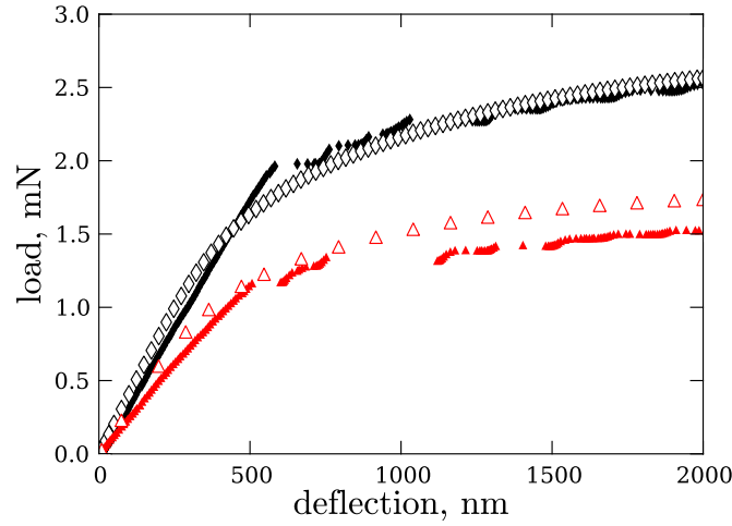
Figure 6.2 Comparison of the experimental load-deflection response of two cantilevers with the notch placed in a single grain (solid symbols) with the corresponding simulation data (open symbols).
