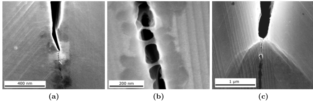
Figure 4.14 (a) Sharp crack tip as observed in most specimens. Slip lines can be seen on one of the adjacent grains. (b) Bridging elements found behind a crack tip of an underaged specimen. (c) Rounded crack tip in a peak-aged specimen showing massive slip on the crack ground.
