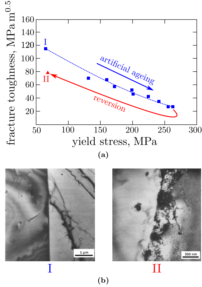
Figure 1.1 (a) Yield stress versus fracture toughness for different heat treatments of an aluminum lithium alloy (figure reproduced from [1]). I marks the reference specimens as quenched and II marks the fully reverted specimens. (b) Representative TEM images from grain boundaries of the specimens corresponding to the heat treatments I and II .
