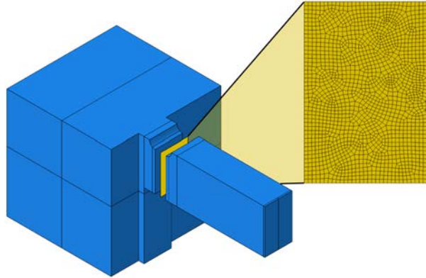
Figure 6.9 Integration of the cohesive zone into the cantilever.
