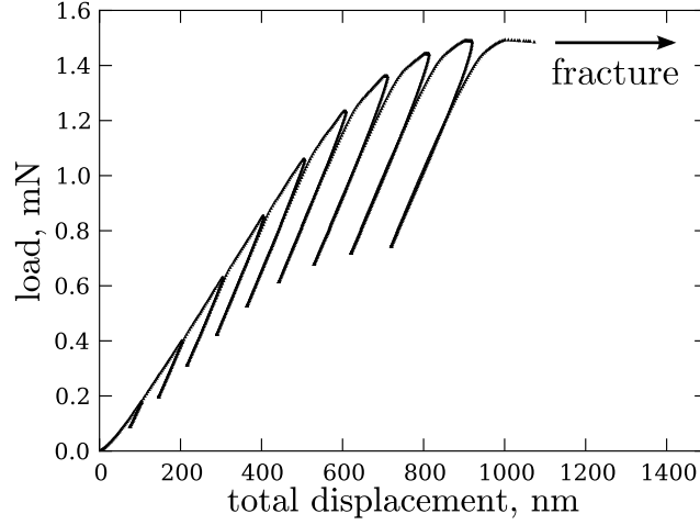
Figure 4.4 Load-displacement data from a typical micro-bending experiment.
