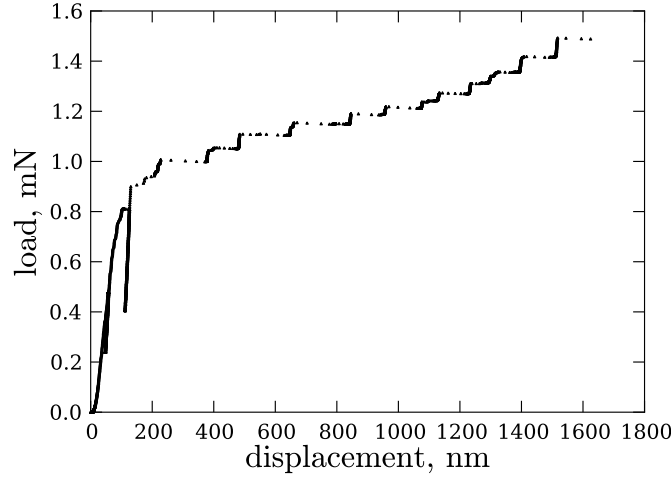
Figure 5.3 Load-displacement response of the micro-column shown in figure 5.2.
