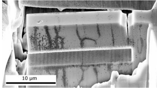
Figure 4.11 Cantilever after the fracture test. The grain boundary under the U-notch failed as desired.
