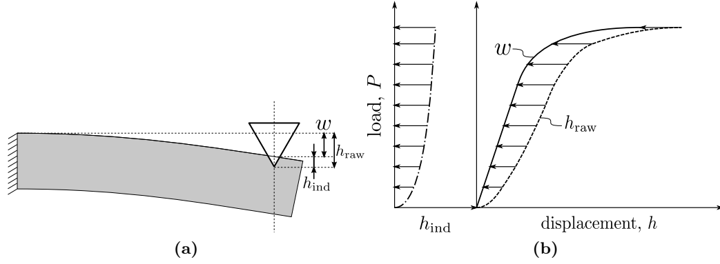
Figure 4.5 (a) Schematic representations of the decomposition of the total measured displacement, h_{\text{raw}} , the cantilever deflection, w , the indentation depth, h^{\text{ind}} , and (b) the correction of the raw data for the indentation depth.
