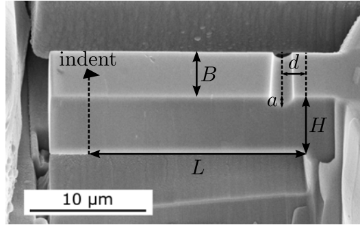
Figure 4.3 SEM image of a cantilever with characteristic dimensions. The dashed line represents a grain boundary. L is the bending length, B is the cantilever width, H is the height of the cantilever, a is the depth of the notch and d is the distance of the notch center to support.
