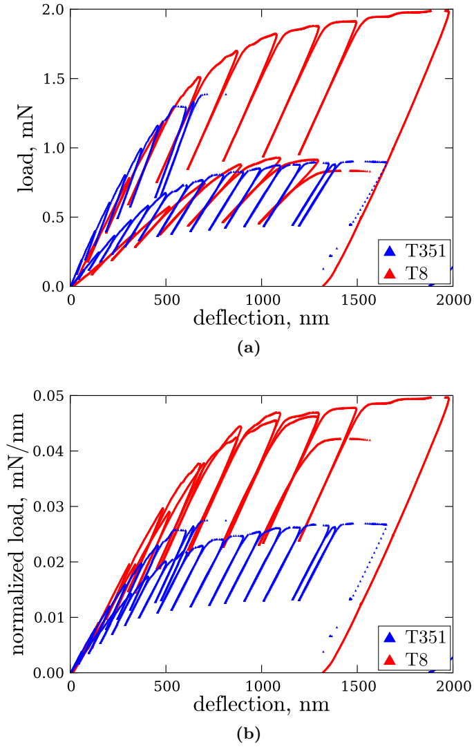
Figure 4.12 (a) load-deflection curves and (b) corresponding normalized load-deflection curves for specimens of the tempers T351 (CB-6, CB-7) and T8 (CB-1, CB-2).
