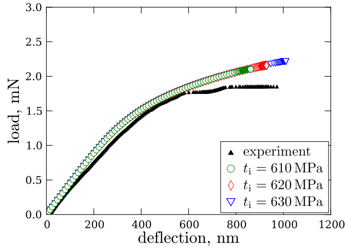
Figure 6.11 Load-displacement data of cantilever A. The cantilever failed at 1000 \pm 50 nm. The initiation stress, t_i has been adjusted to match the displacement at failure while the fracture energy was kept constant at 5 \text{ J/m}^2 .
