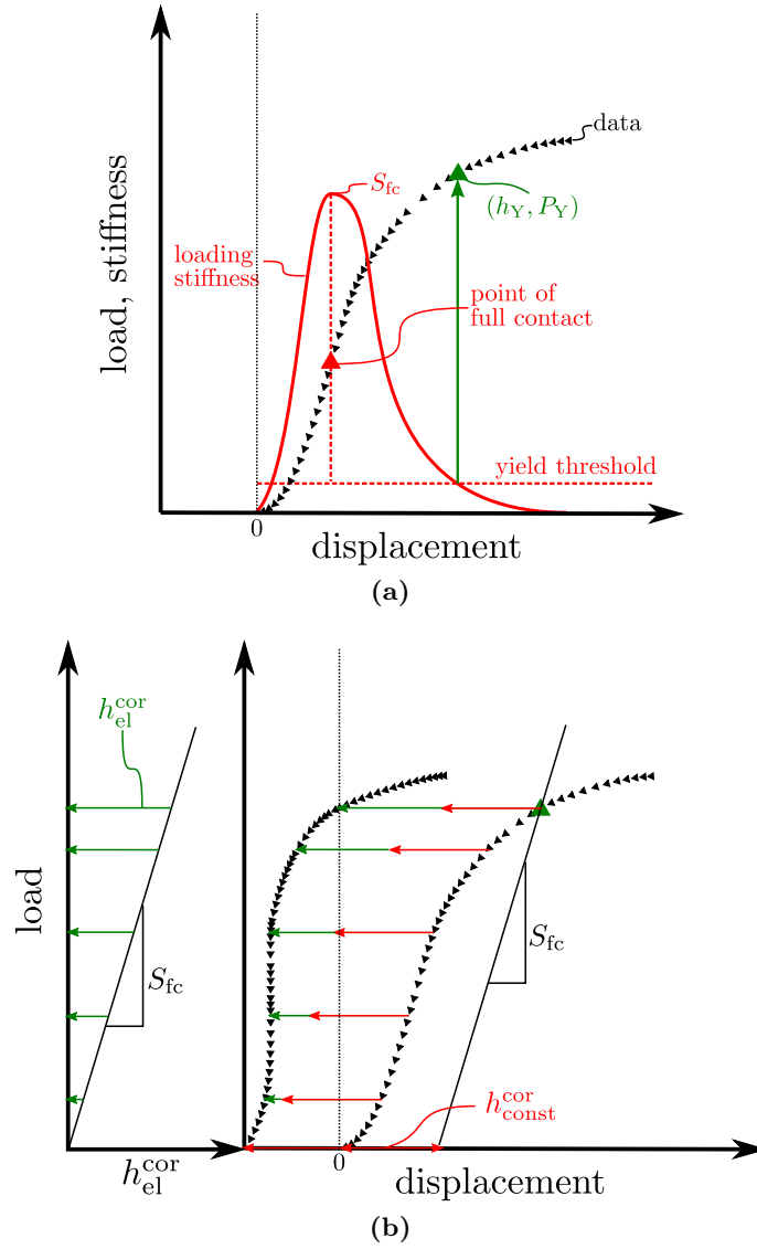
Figure 5.4 (a) Definition of the yield point based on the loading stiffness of a micro-column. (b) Correction to the experimental compression data of a micro-column to obtain the displacement associated with plastic deformation starting at the yield point.
