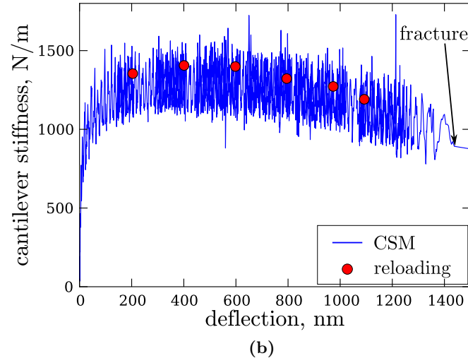
Figure 4.7 Elastic cantilever stiffness measurements of cantilevers with (a) constant stiffness (CB-8) and (b) decreasing stiffness prior to fracture (CB-9). The stiffness measured from reloading segments (red dots), the elastic cantilever stiffness measured by CSM (blue curve) are given for the corrected datasets.
