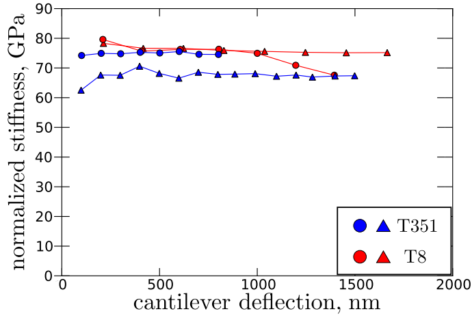
Figure 4.13 Normalized stiffness versus the deflection of the cantilever at the beginning of each corresponding unloading segment.
