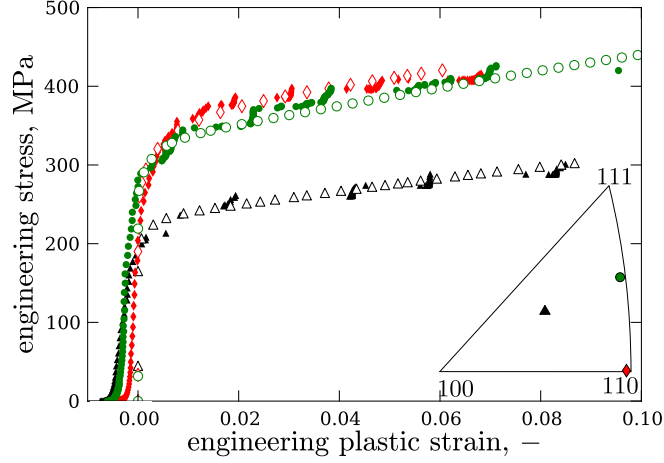
Figure 5.9 Load-displacement response (solid symbols) and FE-prediction (open symbols) for the columns used for the fitting of the crystal plasticity parameters (CC-1, CC-14 and CC-15).
