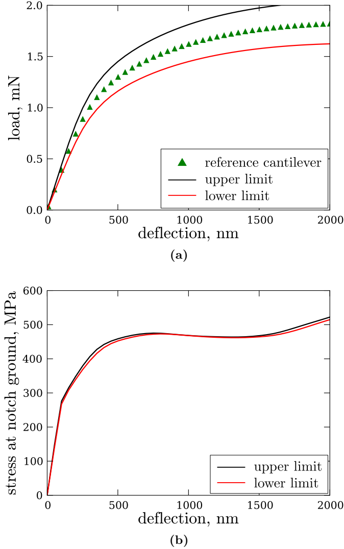
Figure 6.5 (a) Load-deflection response of a cantilever with the dimensions height : width : length = 8.0\text{ }\mu\text{m} : 5.0\text{ }\mu\text{m} : 20.0\text{ }\mu\text{m} together with the upper and lower limits due to deviations in the geometry. (b) Stress at the center of the notch ground for the upper and lower limits.
