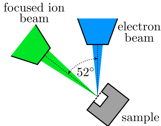
Figure 3.1 Schematic of a combined FIB/SEM system with a sample in the position of the standard milling procedure.
