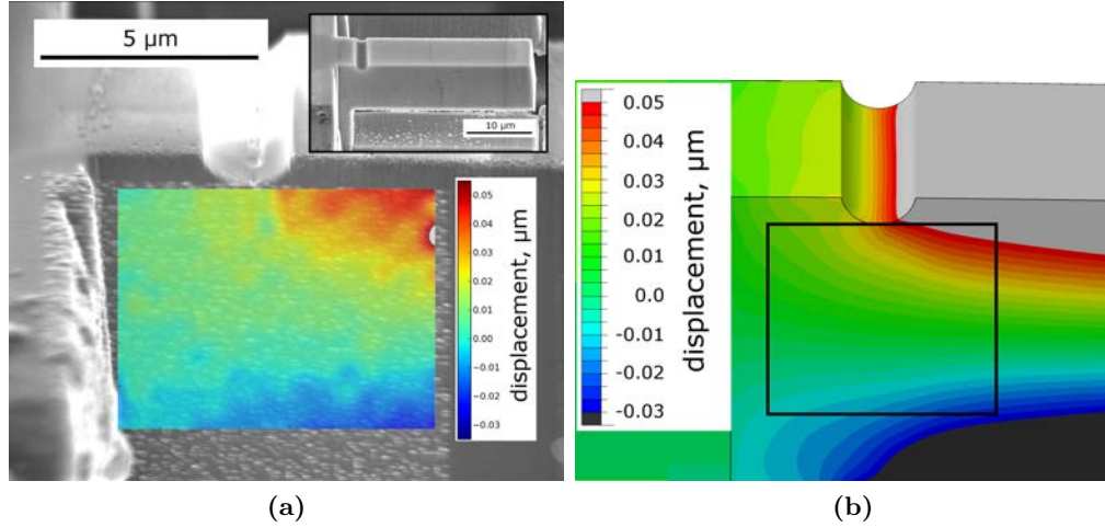
Figure 6.4 Displacement field at the notch ground of a cantilever measured by digital image correlation (a) and extracted from the corresponding FEM simulation at the same load (b).
