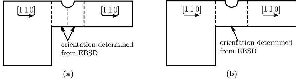
Figure 6.1 Orientations within the cantilever model (a) with the notch at the position of a grain boundary and (b) with the notch placed within a single grain.
