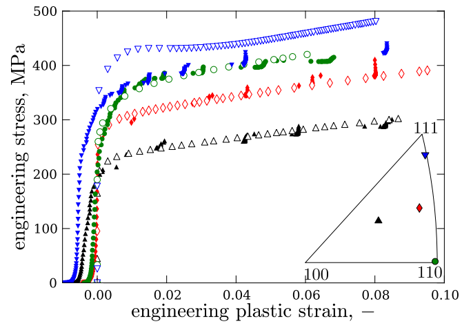
Figure 5.13 Anisotropic yield according to various crystal orientations (solid symbols). Open symbols represent the simulation results.
