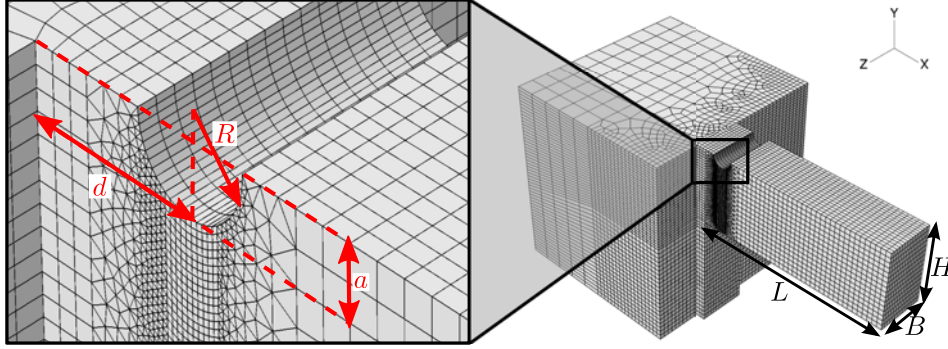
Figure 4.8 Finite element model of a micro-cantilever. The geometric features given are the bending length, L , the width, B , the height, H , the position of the notch center, d , the notch depth, a and the notch radius, R .
