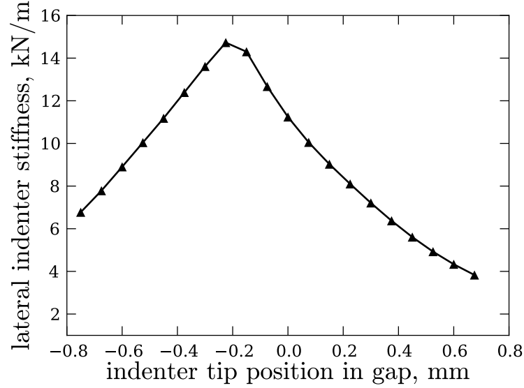
Figure 4.9 Lateral stiffness of the indenter as a function of the position of the indenter tip relative to the load frame.
