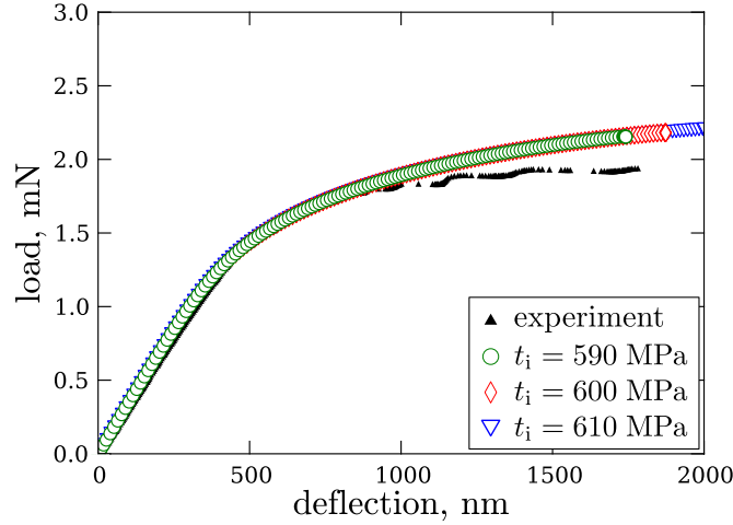
Figure 6.12 Load-displacement data of cantilever B. The cantilever failed at 1800 \pm 50 nm. The initiation stress, t_i , has been adjusted to match the displacement at failure while the fracture energy was kept constant at 5 \text{ J/m}^2 .
