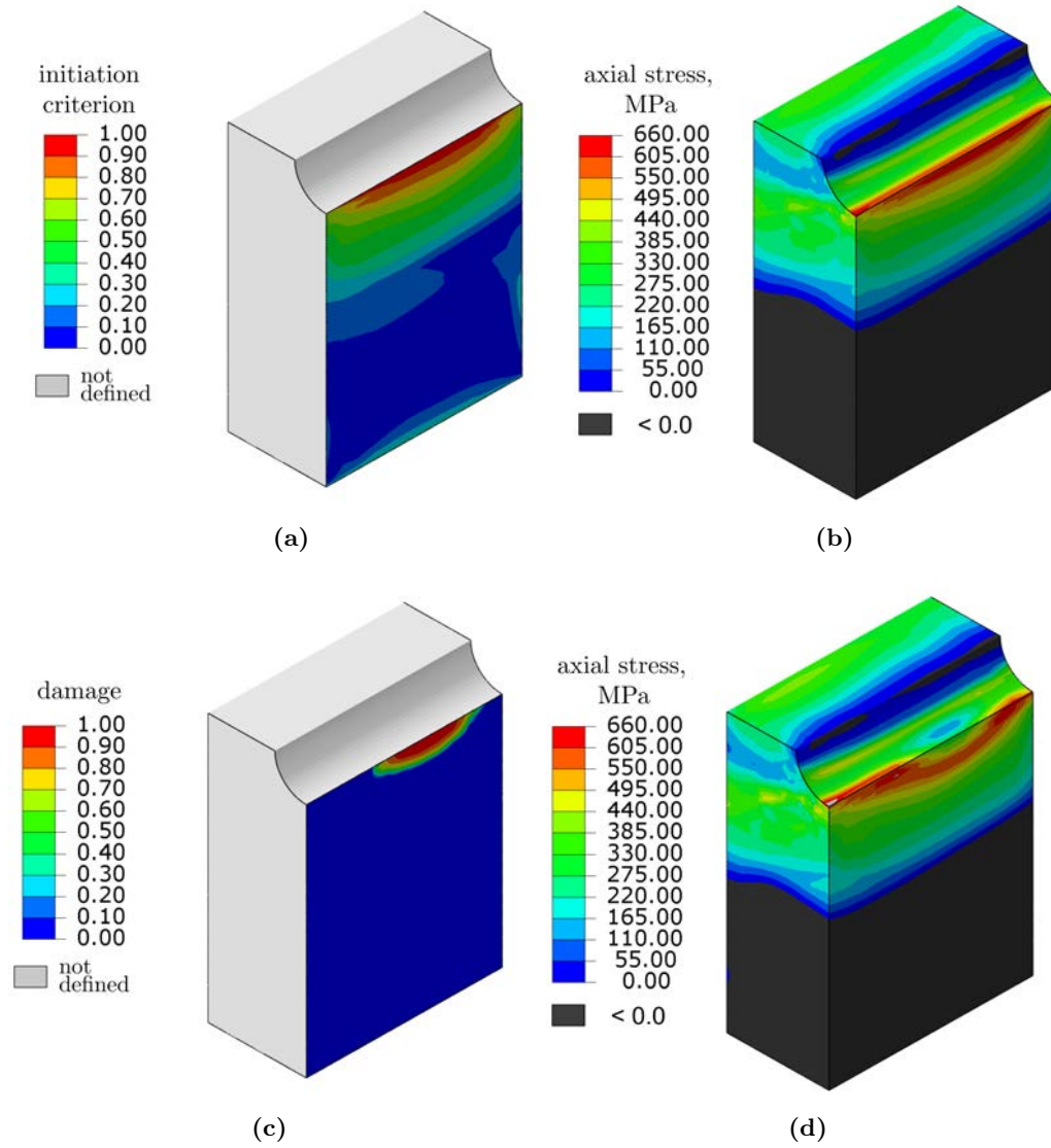
Figure 6.14 Cantilever A: (a) Initiation criterion and (b) stress distribution in the material adjacent to the grain boundary at the moment of initiation. (c) Damage and (d) normal stress distribution at the grain boundary for the last increment of the simulation.
