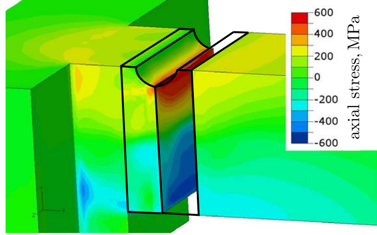
Figure 6.7 Normal stress along the cantilever axis at the grain boundary at the fracture load predicted by a finite element simulation.
