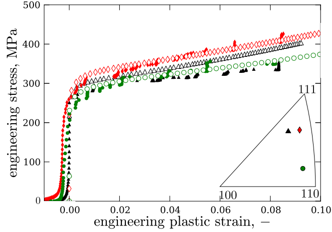
Figure 5.10 Examples for the application of the calibrated crystal plasticity model to columns with various orientations (CC-3, CC-7 and CC-17). Solid symbols are experimental data, open symbols represent simulation data.
