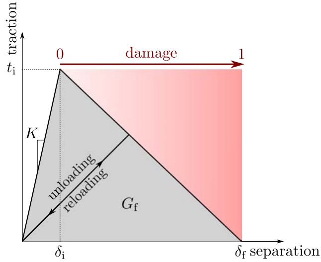
Figure 6.8 Representation of the traction-separation law applied within the present work.
