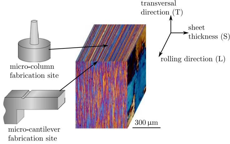
Figure 4.1 Microstructure of the AA2198 sheets after Barker's etch ( \text{HBF}_4 + \text{H}_2\text{O} , anodized using 0.2 A/cm 2 ), observed in polarized light.
