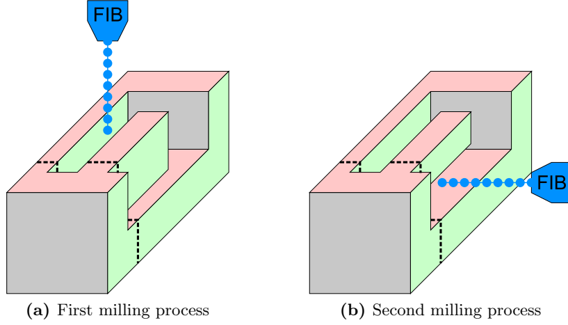
Figure 4.2 Preparation of a cantilever from the edge of a sample.
