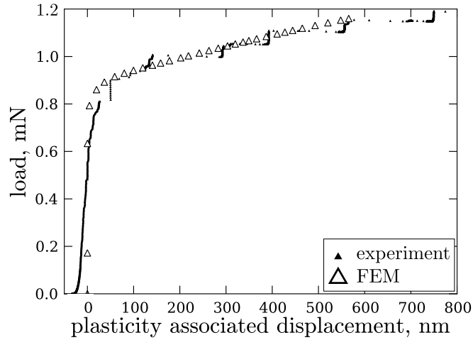
Figure 5.6 Load-displacement response of the specimen oriented for single slip (CC-1). Open symbols represent the simulation results, solid symbols give the experimental data.
